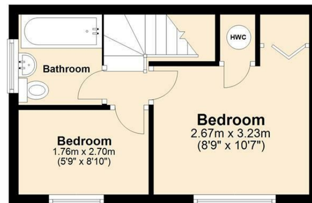
First Floor Approx. 22.6 sq. metres (242.9 sq. feet)
